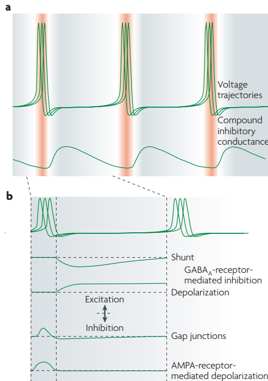
Figure 6 | Several synaptic mechanisms underlie synchronization in interneuron networks during gamma oscillations.
